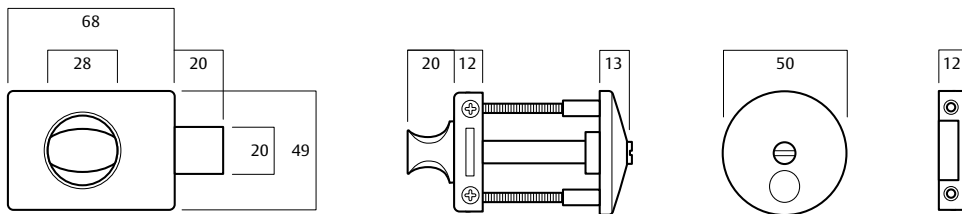
Toilet bolt with indicator (emergency release)
