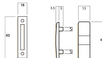
Flat keeper
