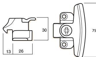
Lockable
