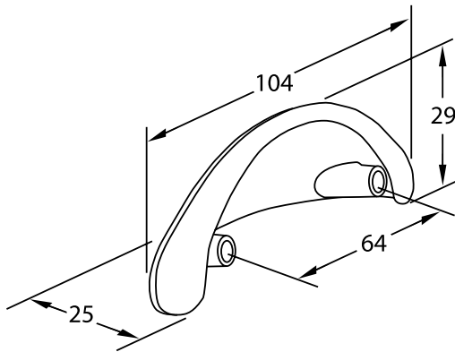
Cup Pull Part no. CTCP
