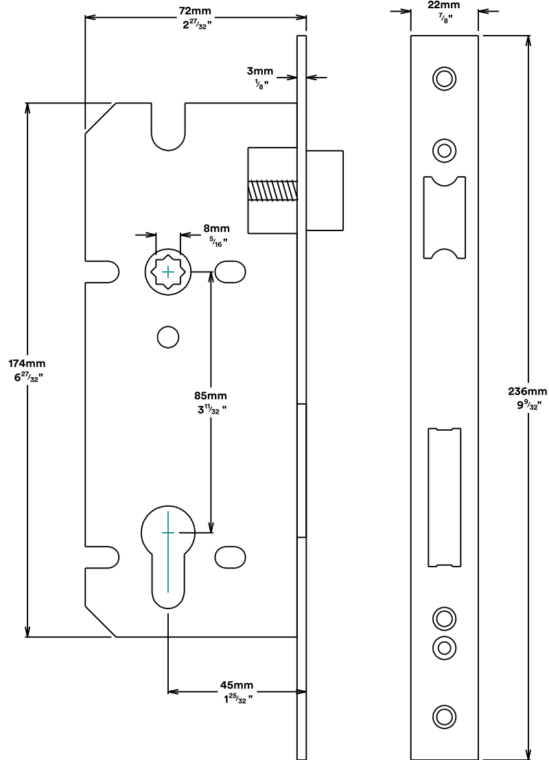
Mortise Lock & Faceplate
