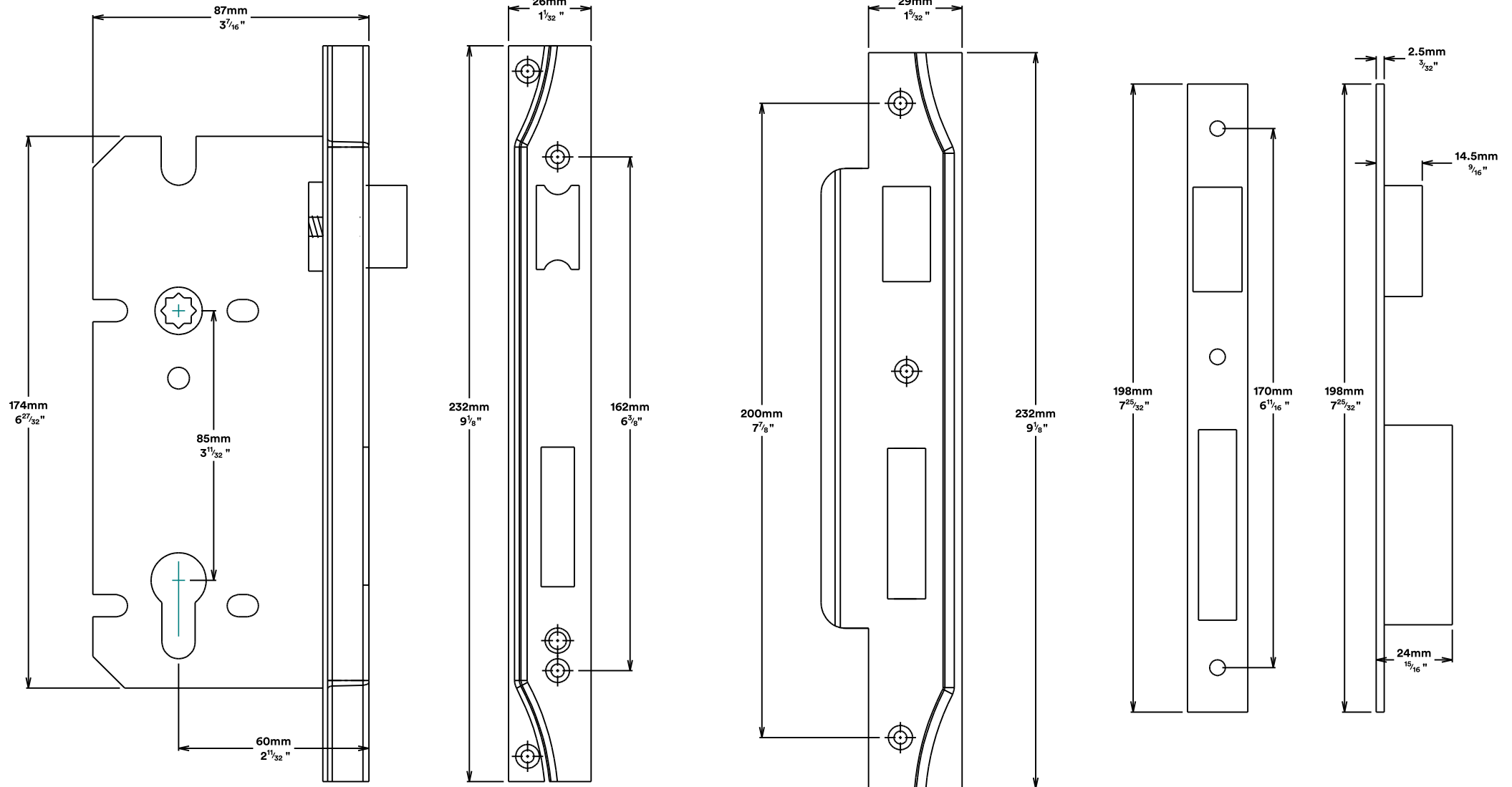
Mortice Lock & Rebated Face plate
