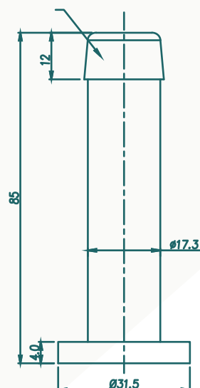
RUBBER CAP
