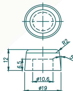
RUBBER STOPPER
